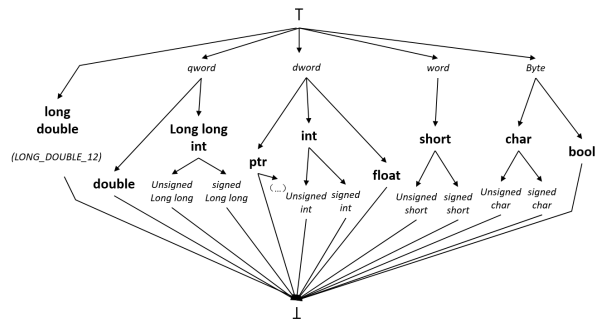
Fig. 10. Type Lattice for Hex-Rays and BITY
